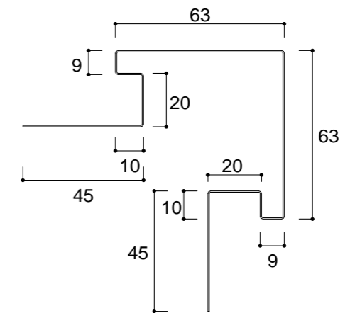
NK - 300 (横張用・出隅) L = 2000 ~ 3000
