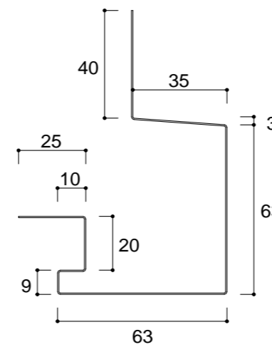
NK - 150 (天井正面接続) L = 2000 ~ 3000
