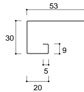
NKR - 101 (廻り縁) L = 2000 ~ 3000
