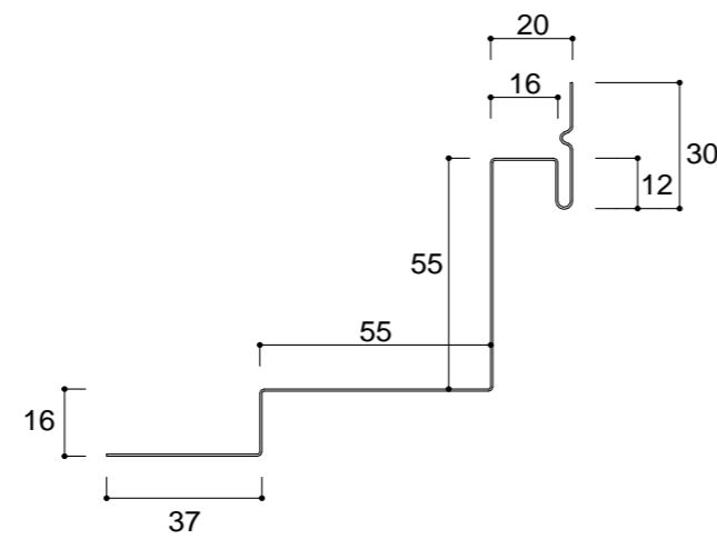
NKR - 304 (入隅) L = 2000 ~ 3000
