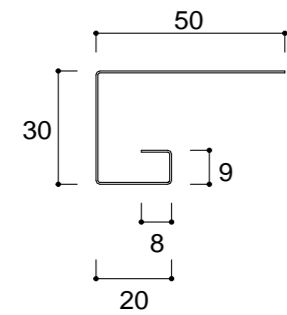
NK - 101 (廻り縁) L = 2000 ~ 3000
