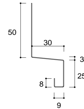
NK - 300 (横張用・出隅) L = 2000 ~ 3000
