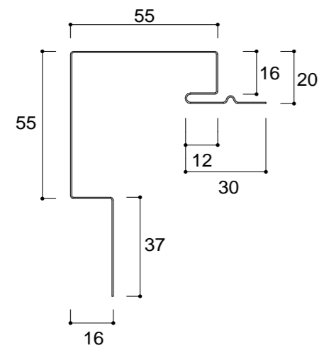
NKR - 303 (出隅) L = 2000 ~ 3000
